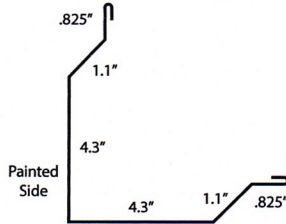
Outside Corner Length 10'2"
