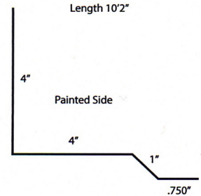
Transition (Lower Gambrel) Length 10'2"
