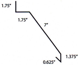
Cannonball Track Cover Length 10'2"
