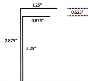
Gutter Apron Length 10'2"
