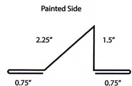
Upper Gambrel Length 10'2"
