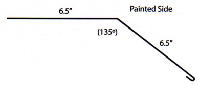
Upper Gambrel Length 10'2"
