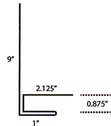
Rat Guard (Base Angle) Length 10'2"
