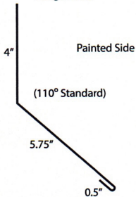
F&J For Soffit Length 10'2"
