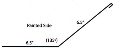
Transition (Lower Gambrel) Length 10'2"
