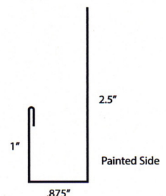
J-Trim Length 10'2"
