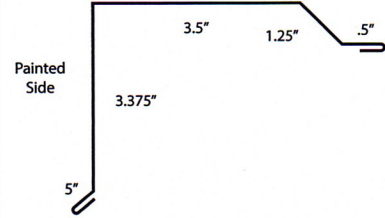
Denver Rake Length 10'2"
