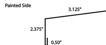
Gutter Apron Length 10'2"
