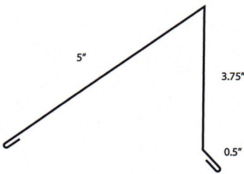
Ridge Cap Length 10'2"
