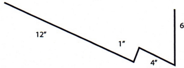
Drip Cap Length 10'2"
