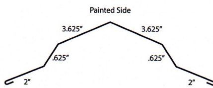
Ridge Cap Length 10'2"
