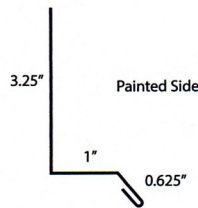
Drip Cap Length 10'2"
