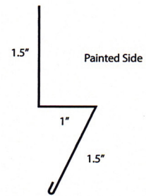
Snowguard Length 10'2"
